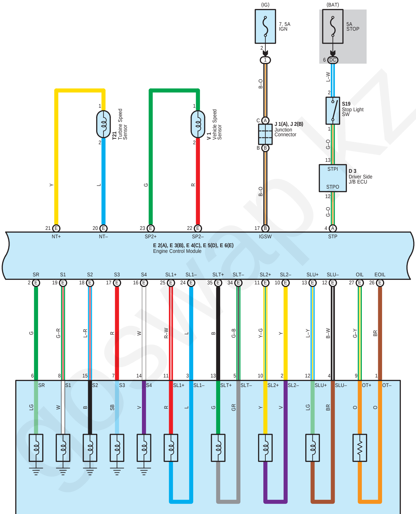
E 1 Electronically Controlled Transmission Solenoid
